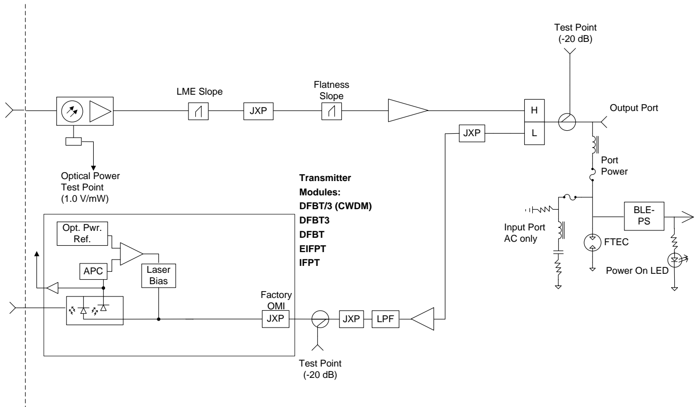
BLN100 Block Diagram
